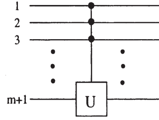
Fig. 1. The network notation for \Lambda_m(U) ; see Definition 1 for \Lambda_m(U) .
