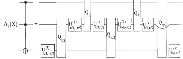
Fig. 7. The network simulating the Toffoli gate using the basic gates U_{\theta, \phi} and Q_\eta .
