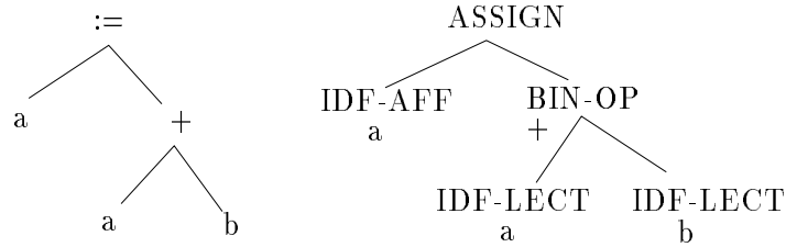
Figure 14: Parse tree of the instruction "a:=a+b". On the left side: the parse tree is labeled with words of the PASCAL program. We will use another format described on the right. The labels are made of two parts: the first part specifies the kind of the node, the second part is an attribute. For example, IDF-AFF indicates that the node contains the name of a variable that is modified, IDF-LECT : the name of a variable which is read, BIN-OP the name of a binary operator like the addition, ASSIGN corresponds to an assignment. For nodes IDF-AFF and IDF-LECT , the attribute contains the name of the variable to modify or to read. For BIN-OP , the attribute contains the name of the particular binary operator.
