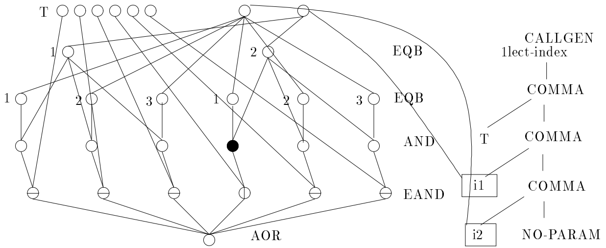
Figure 43: Reading of a 2D array [0..1][0..2] of integers. The index i1 is 2, the index i2 is 1. The two first layers of neurons EQBs have a sigmoid that test the equality to zero. They output 1 if the net input is 0, otherwise they output -1. These EQB neuron's threshold are indicated. The third layer of neurons computes logical ANDs . In this layer, a single neuron outputs 1, the one that corresponds to the element that must be read. All the other neurons of this layer output -1. The fourth layer of neurons is a layer of EAND neurons. only one of these neuron is activated. It propagates the element of the array that is read. Last, a neuron AOR merges all the output lines and retrieves the element that is read. The instruction CALLGEN is almost like CALL-F , except that all the links to the global variables are deleted. CALLGEN is described in the next to the next figure.
