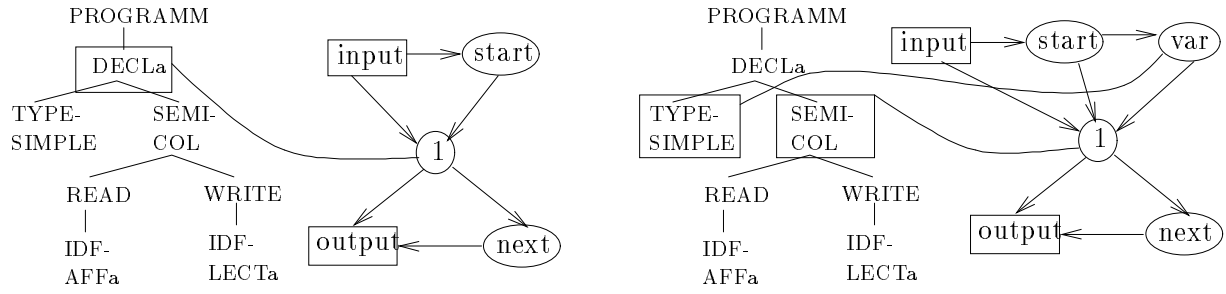
Figure 23: On the left: execution at step 1 of the macro program symbol PROGRAM . The ancestor cell “1” gives birth to two other cells. A cell labeled “start” and another one labeled “next”. The “start” cell controls the propagation of the activities. The “next” cell has not finished its development. It waits all its neighbors to become finished neurons. The cell “1” now reads the DECL node. On the right: execution at step 2 of the macro program symbol DECL . The ancestor cell gives birth to another cell labeled “var”. This cell represents the variable “a”. The input and output connections of the ancestor cell are now complete and represent a topological invariant. The first input (resp. output) link points to the input (resp. output) pointer cell. The second input link points to the “start” cell, the rest of the input links point to “var” neurons. The second output link points to the “next” cell.
