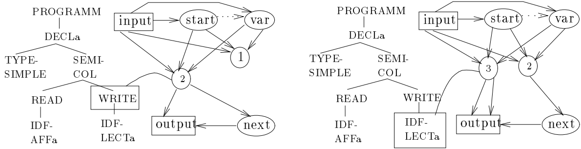
Figure 26: On the left: unblocking at step 7 of the cell “2”. Before to start the compilation of the WRITE , cell “2” executes a small piece of cellular code. It merges the input links of cell 1. The cell “1” will be deleted. Now, the invariant is restored. Cell “2” can start the compilation of the next instruction. On the right: execution at step 8 of the macro program symbol WRITE . The cell “2” gives birth to another cell “3”, connected two times to the output pointer cell. The cell “3” possesses all the input connections of cell “2”. Cell “2” becomes a neuron.
