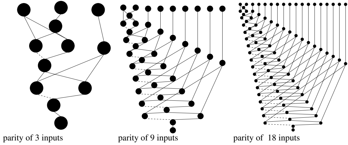
Figure 8: The final decoded neural network that computes the even parity of 3, 9 and 18 binary inputs. The initial life is respectively 2,8 and 17. A weight -1 is represented by a dashed line. With an initial life of L we develop a neural network for the L + 1 input parity problem, with L copies of the XOR network.
