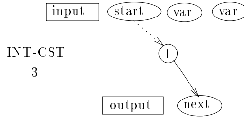
Figure 29: Execution of the macro program symbol INT-CST by the ancestor cell of the invariant pattern. This macro program symbol has one parameter which is the value of the constant. The macro program symbol INT-CST 3 has the following effect: It sets the bias of the ancestor cell to the value 3, and deletes all the links, except the link to the “start” neuron and the link to the “next” neuron. The sigmoid of the ancestor cell is set to the identity, and the ancestor cell becomes a neuron labeled 1. When the constant is needed, the neuron “start” is used to activate the neuron 1, which delivers the constant coded in its bias.
