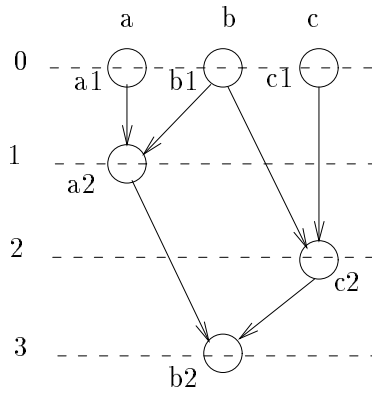
Figure 13: Result of the compilation of the PASCAL program: var a,b,c: integer; begin a=a+b; c=c+b; b=a+c; end. Each dotted line corresponds to the compilation of one instruction. The neurons make a simple addition of their inputs (the weights are 1, the sigmoid is the identity). The line 0 represents the initial environment. It encompasses three values “a”, “b” and “c” stored in three neurons a_1 , b_1 and c_1 . At line 1, the value of “a” has changed, it is now contained in a new neuron a_2 , that computes the sum of “a” and “b”. In order to make this sum, neuron a_2 is connected to neuron a_1 and b_1 . The value of “c” changes at the next line, finally, the value of “b” also changes. One can see that the two first instructions: a:= a+b; c:=c+b can be executed in parallel by neurons a_2 and c_2 . On this example, each variable is represented by two neurons during the run of the program.
