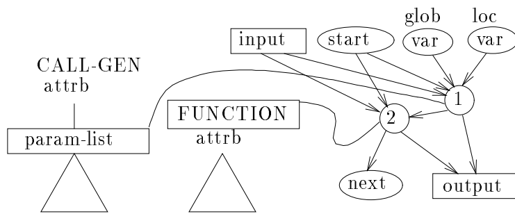
Figure 45: Execution of the macro program symbol CALLGEN by the ancestor cell of the invariant pattern. CALLGEN has the same effect as CALL-F except that the cell “2 ” which will execute the body of the function written in cellular code, does not have connections to the global variables of the PASCAL program.
