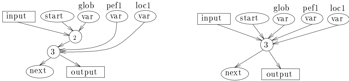
Figure 35: Execution of the cellular code RESTORE by cell “3” of the preceding figure. Cell “3” is unblocked when the body of proc2 is developed. Cell “3” is linked to cell “2” which is linked to the global variables, that may have been modified by the called procedure. The execution of RESTORE brings together the modified global variables, and the unchanged local variables of proc1 .
