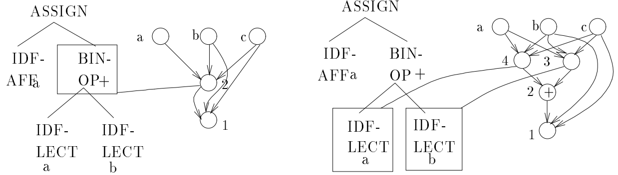
Figure 16: On the left: execution at step 2 of the macro program symbol IDF-AFF , read by the cell "1". Cell "1" deletes its first link, and moves its fourth link back in the first position. On the right: execution at step 3 of the macro program symbol BINOP read by cell "2". Cell "2" divides into three cells "2", "3" and "4". Cells "3" and "4" inherit the input links of their mother cell, and are connected on the output to cell "2". Whereas cell "2" inherits the output links of the mother cell, loses its reading head and becomes a neuron. The sign + inside the circle indicates that it makes the addition of its inputs.
