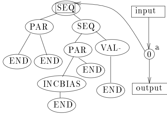
Figure 2: Step 0: Development of the neural net for the exclusive-OR (XOR) function in the right half of this figure. The development starts with a single ancestor cell labeled "a" and shown as a circle. The 0 inside the circle indicates the threshold of the ancestor cell is 0. The ancestor cell is connected to the neural net's input pointer cell (box labeled "input") and the neural net's output pointer cell (box labeled "output"). The cellular encoding of the neural net for XOR is shown on the left half of this figure. The arrow between the ancestor cell and the symbol SEQ of the graph grammar represents the position of the reading head of the ancestor cell.
