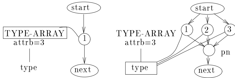
Figure 41: Execution of the macro program symbol TYPE ARRAY . This macro program symbol develops the neural tree of pointer neurons that is required to encode an array. We need d macro program symbols TYPE ARRAY in order to represent an array of d dimensions. TYPE-ARRAY has one parameter which is the number of columns along the associated dimension.
