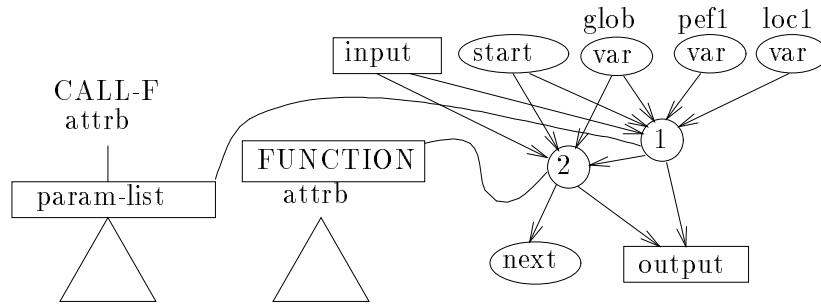
Figure 38: Execution of the macro program symbol CALL-F by the ancestor cell of the invariant pattern. This macro program symbol has the same effect as CALL-P except that it does not create the cell 3, because it is not necessary to restore the environment.
