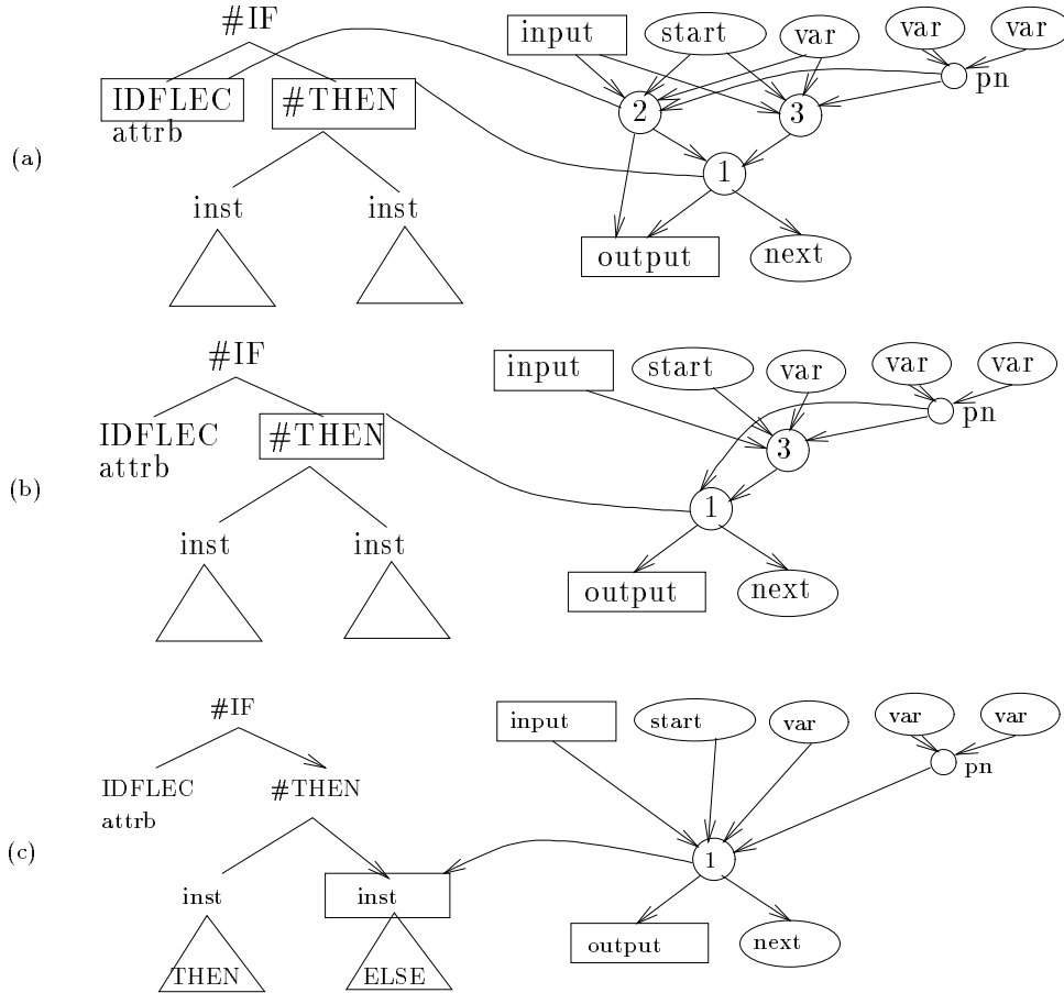
Figure 46: On the top (a): execution of the macro program symbol #IF by the ancestor cell of the invariant pattern. Three cells are created. Cell “2” goes to read a macro program symbol IDF-LEC that will select the array variable which is concerned by the test. Cell “3” is a neuron that will be used later by cell “1” to restore the environment, once the test is finished. On the middle (b): execution of the macro program symbol IDF-LEC , by cell number “2” of the preceding figure. On the bottom (c): execution of the macro operator #THEN by cell “1”. Cell “1” tests the number of input links of its first neighbor. Here this number is 2 because the array has two elements. If this number is greater than one, cell “1” places its reading head on the right subtree, as it is the case here. Otherwise it goes to read the left subtree. Finally, cell “1” merges the links of the neuron “3”.
