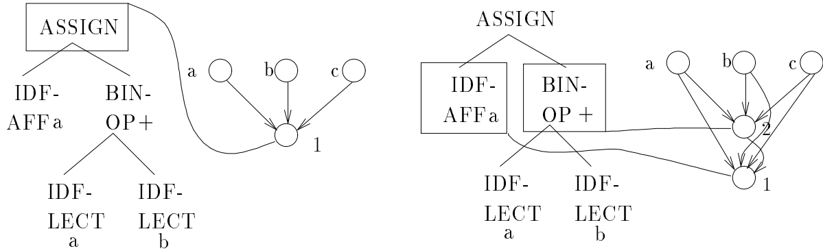
Figure 15: On the left: Development of the neural network translating the PASCAL instruction "a:=a+b". The development begins with an ancestor cell labeled "1" connected to three neurons labeled "a", "b" and "c" which store the state of the environment before the instruction is executed. On the left side, we represent the parse tree of the PASCAL instruction. The arrow between the ancestor cell and the symbol ASSIGN of the parse tree represents the reading head of the ancestor cell. On the right: execution at step 1 of the macro program symbol ASSIGN , read by the ancestor cell "1". Cell "1" divides into two child cells "1" and "2". Both child cells inherit the input links of the mother cell. Child "2" is connected to child "1". The reading head of cell "1" now points to the node IDF-AFF and the reading head of cell "2" points to the node BIN-OP
