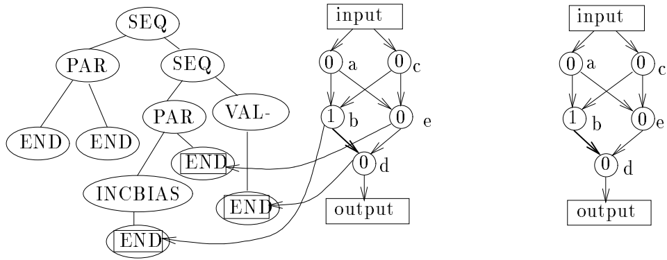
Figure 6: On the left: Neuron "b" executes the value-program symbol INCBIAS . The action of INCBIAS is to increase the threshold of cell "b" by 1. After execution, the threshold of cell "b" is 1, and the reading head of cell "b" points to an END at the fifth level of the tree. On the right: The last tree steps consist in executing three END -program symbols. The three END 's cause the cells "b", "e" and "d" to lose their reading head and become finished neurons. Since there are now only finished neurons, the development is finished. The final neural net has two input units "a" and "c", and one output unit "d". The neuron "c" is the second input unit, because the link from the input pointer cell to "c" is the second output link of the input pointer cell
