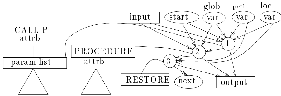
Figure 34: Execution of the macro program symbol CALL-P by the ancestor cell of the invariant pattern. The environment has three variables. The CALL-P has one parameter ( attrb ) which is the name of the called procedure. Three cells are created. Cell “1” develops different subnetworks: one subnetwork for each parameter to pass to the called procedure. The cell “2” develops the body of the called procedure. Its reading head is placed on the root of the parse tree that defines the called procedure. The cell “2” is not connected to the neurons that contain the local variables of the calling procedure: pef1 and loc1 . These variables cannot be accessed from proc2 . Cell “3” is blocked on a cellular code RESTORE . It will restore the environment of the calling procedure, when the translation of the called procedure is finished.
