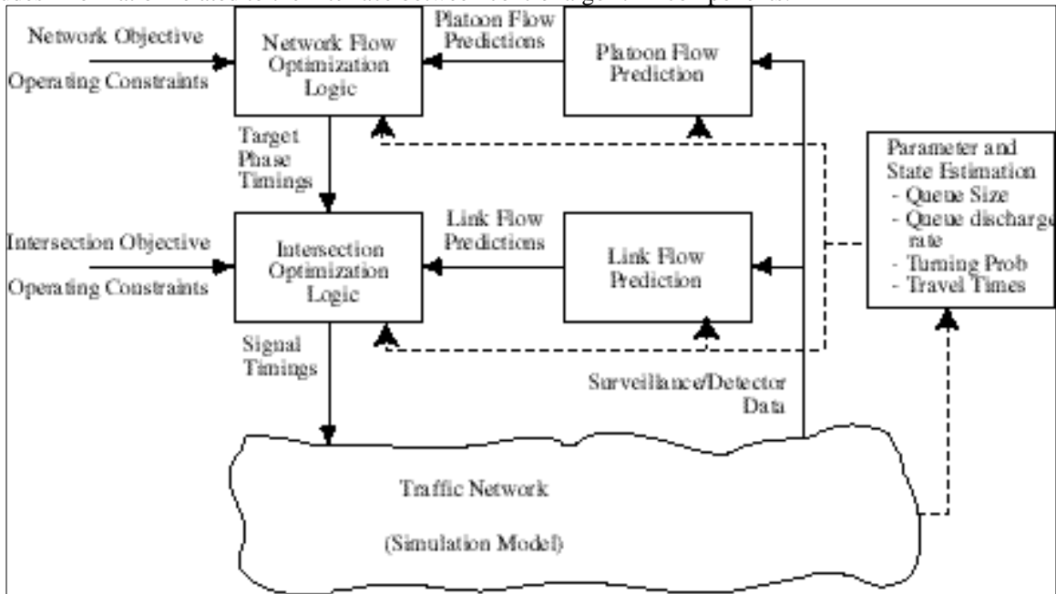
Figure 9. Components of the RHODES Prototype.
