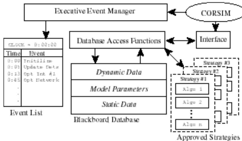
Figure 10. Software Architecture.
