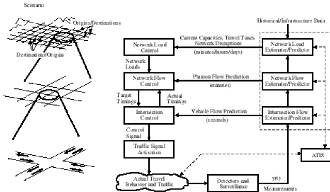
Figure 1. The RHODES Hierarchical Architecture.
