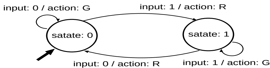
Figure 23: Yet another example of FSM. How do you think its behavior?
