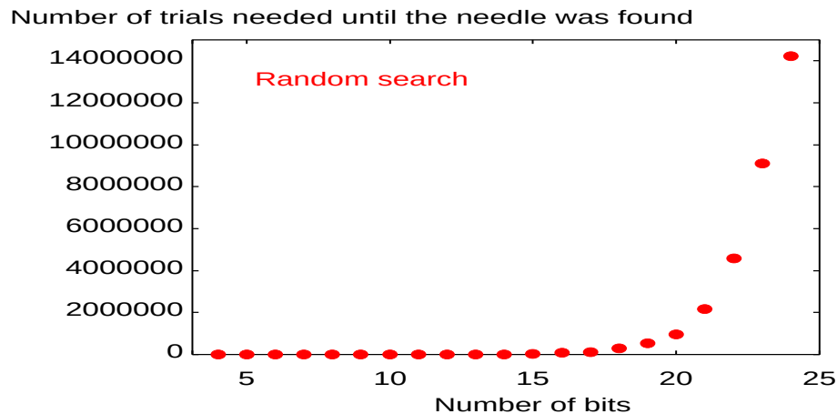
Figure 33: Search will explode exponentially as number of bits grows.
