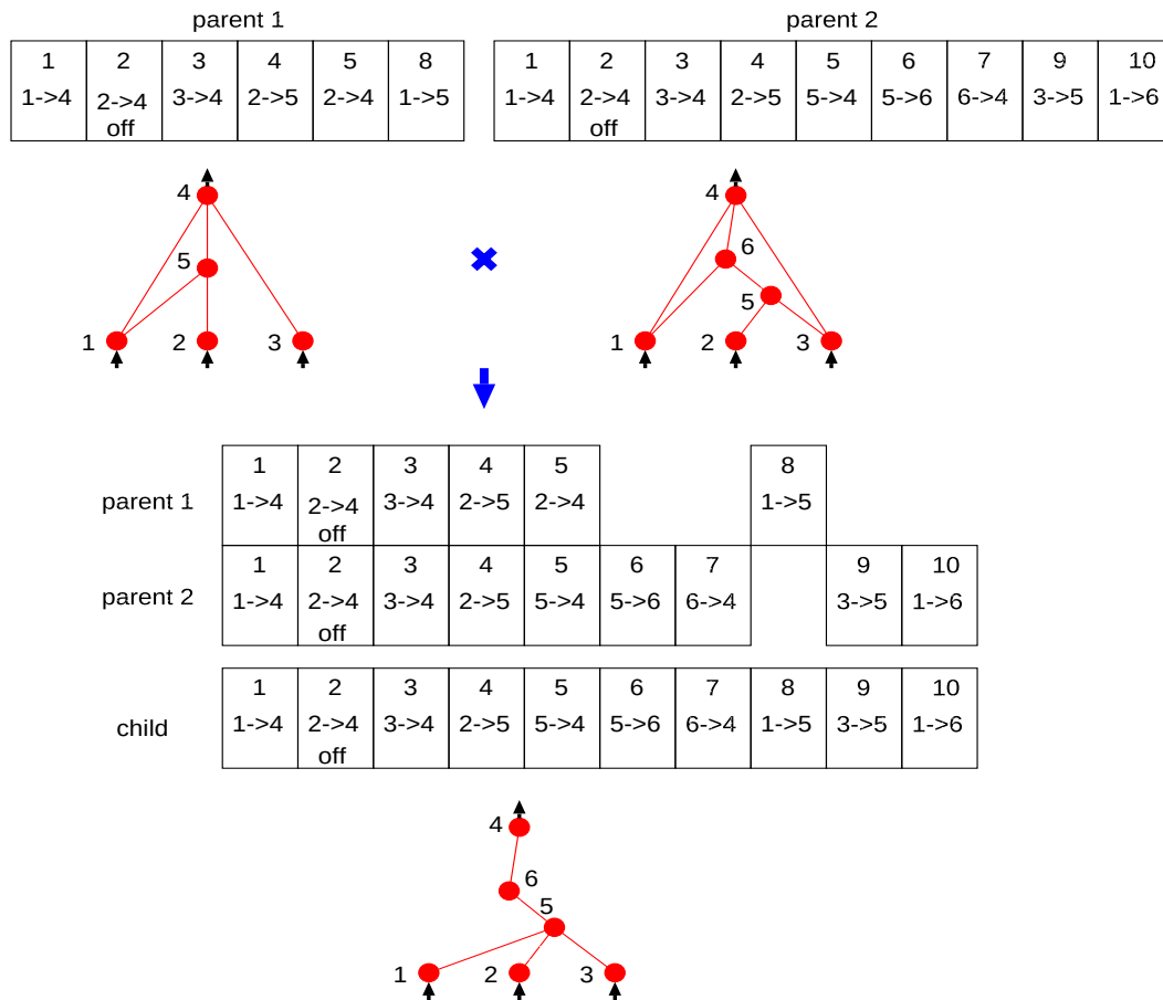
Figure 31: A crossover in NEAT. (Re-drawn the figure in Stanley et al.)
