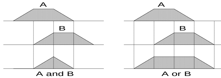
Figure 39: AND and OR in fuzzy set.
