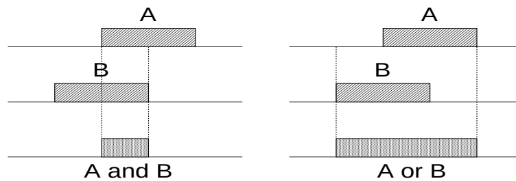
Figure 38: AND and OR in crisp set.
