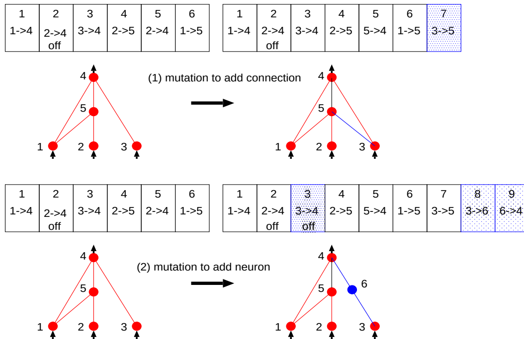
Figure 30: Two types of mutation in NEAT. (Re-drawn the figure in Stanley et al.)
